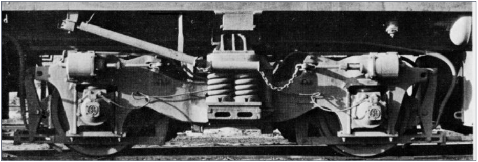
6. In late 1965, Alco offered this high-adhesion two-axle truck on its Century series C415 center-cab heavy switcher. It was also used as an extra-fare option on Alco's high horsepower C430 road switchers introduced in 1966. Note the chain and chain-tubes for the hand-operated parking brake.
