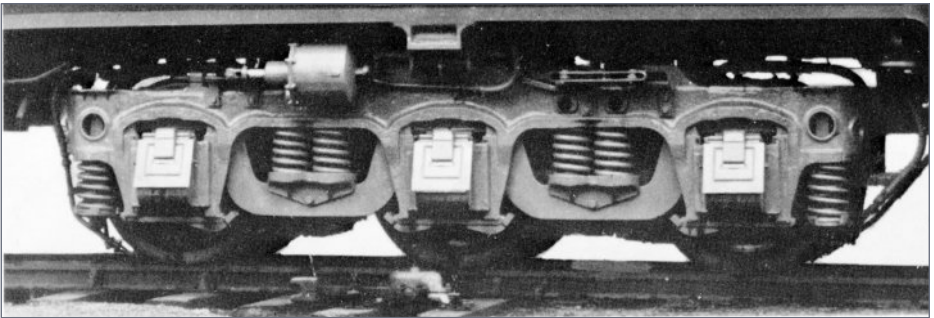
7. Alco used this A1A freight truck on its early DL-109 cab unit introduced in 1941. Note the plain bearing journals, inside drop equalizers, and secondary equalizer springs at both ends of the frame. This truck was also used on Alco's RSC-2 and -3 road switchers.
