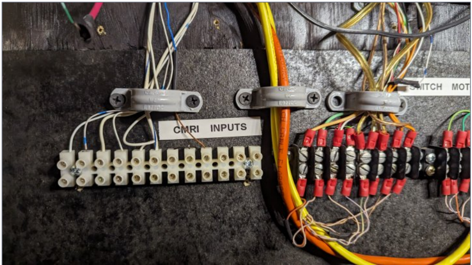
6. European style (left) vs. barrier (right) terminal strip/blocks.
