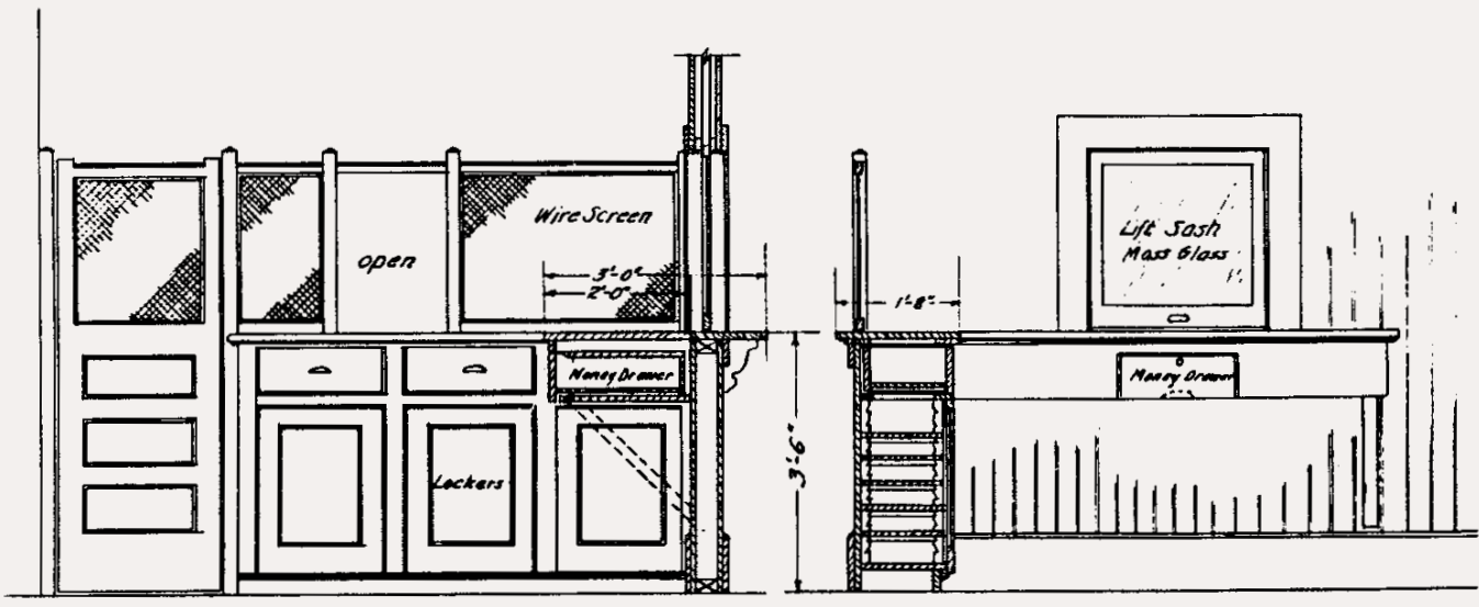
DETAIL OF COUNTER & COUNTERSHELF
