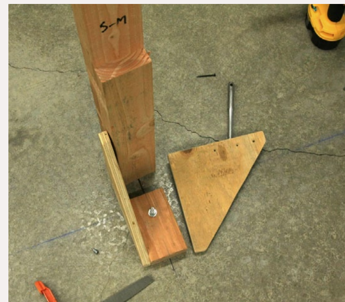
FIGURE 13: Installing a 4x4 leg for the peninsula using a concrete anchor to fasten it to the floor.
